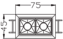
Cutout: L68xW37mm
