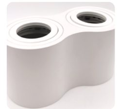
Size: L160xW80xH85mm
